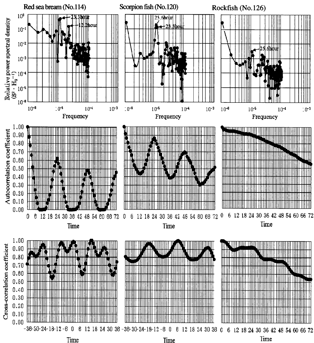
Fig. 14 An example of periodic behavior analysis of three tracking species by stand type.
