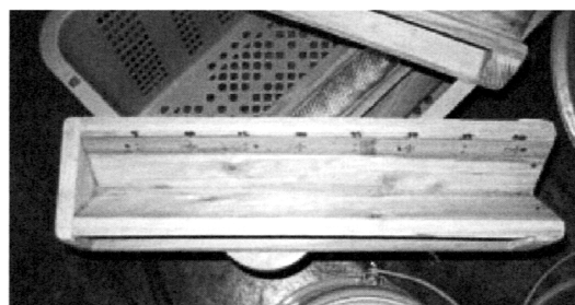
Fig. 5 Insert the pinger, the V-shaped tray for surgery.
