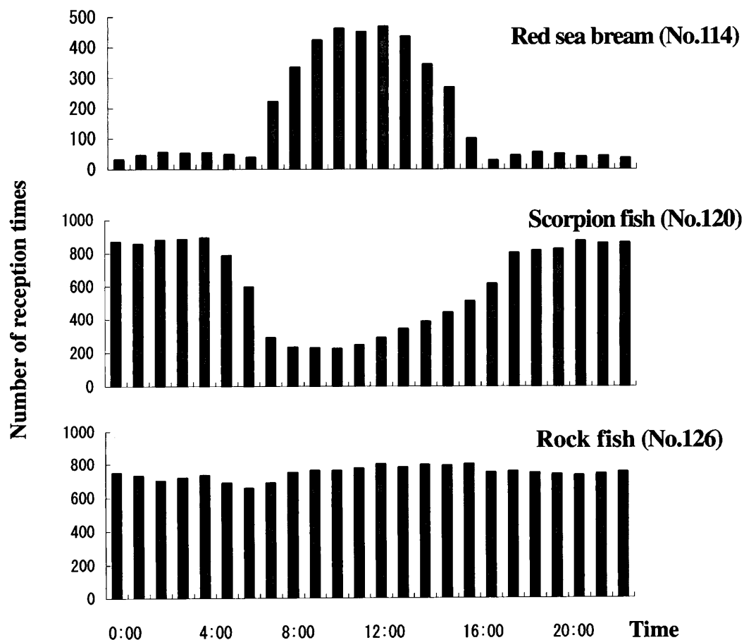
Fig. 13 An example of the activity of three tracking species by stand type at night and day respectively. (70 days) ID numbers in the figure indicate the number of coded pinger.
