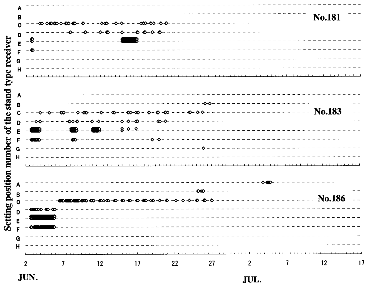
Fig. 8 An example of moving of the jack mackerel between the reefs (2009).
