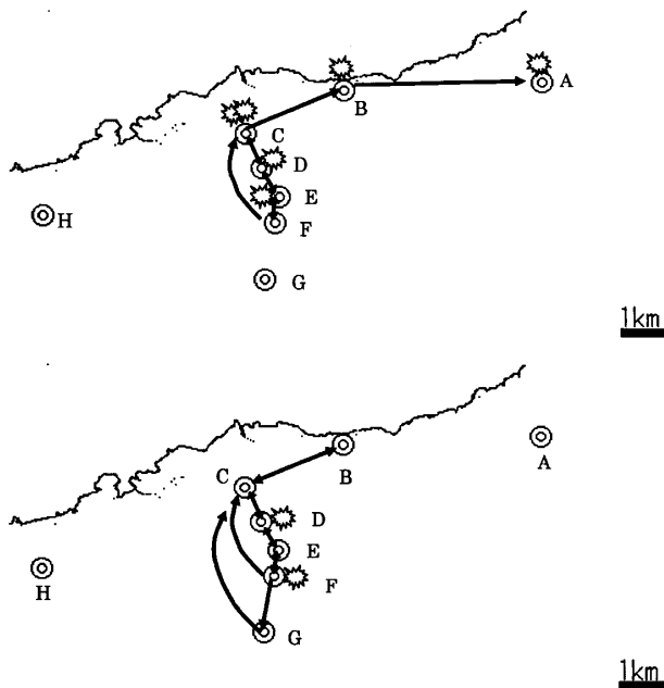
Fig. 9 An example of tracking the jack mackerel for 70 days by stand type receivers.
