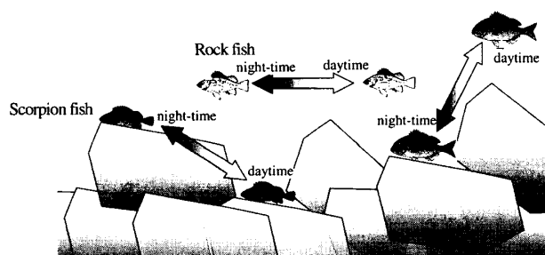
Fig. 15 The moving patterns of the red sea bream, the scorpion fish, and the rockfish in the stone reefs at Harima-Nada and sight frontage of Ieshima.
