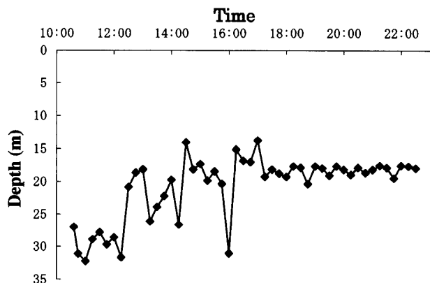
Fig. 11 An example of change of the red sea bream's swimming depth. (Oct.29, 2009, 12 hours)
