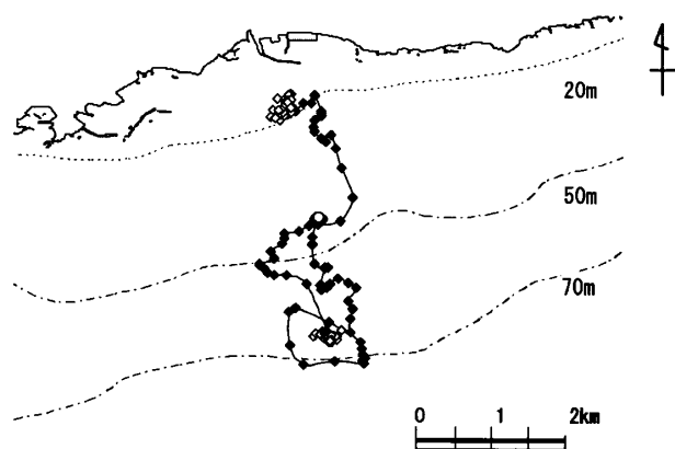
Fig. 6 An example of moving of the jack mackerel between the reef by the tracking type. (Reference from Journal of Fisheries) 7) .
