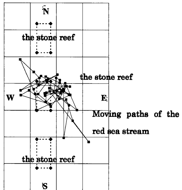
Fig. 10 An example of behavior of the red sea bream by the tracking type (Oct.29, 2009, 12 hours).
