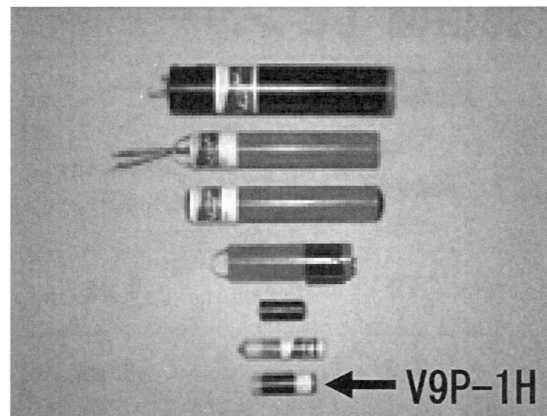
Fig. 2 The shape of pingers (manufactured by Vemco).
