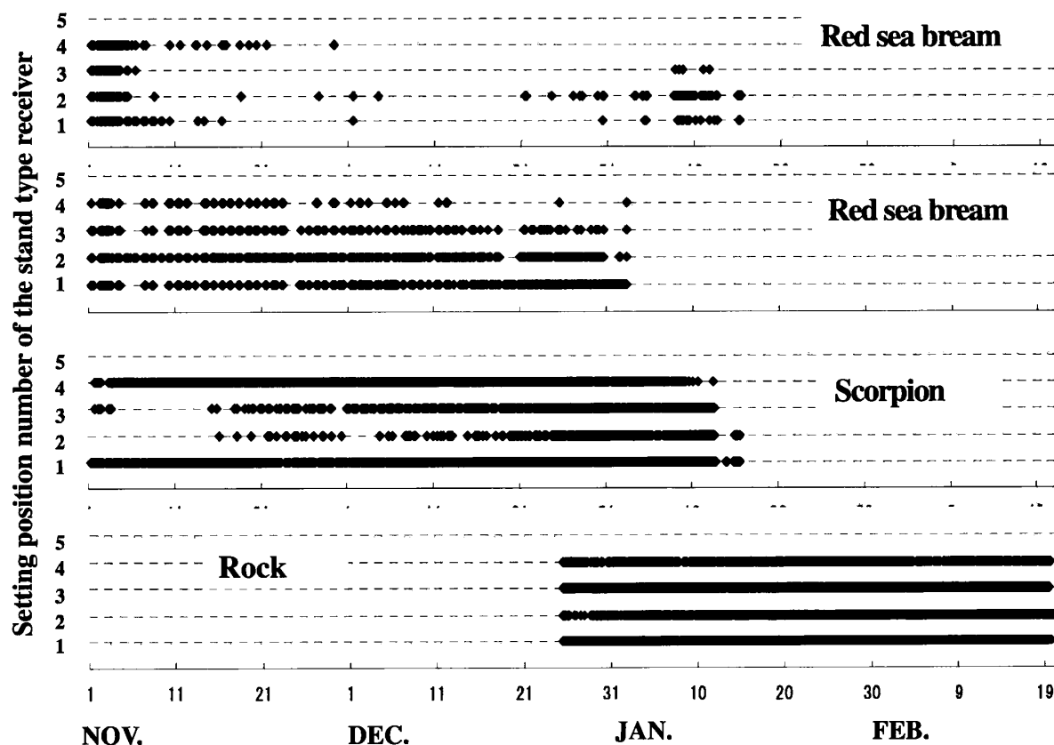
Fig. 12 An example of moving of three tracking species by stand type between the reefs (2009). No.5 lacked. No.1-No.5 in the figure indicate the number of the stand type receiver at Harima-Nada area.
