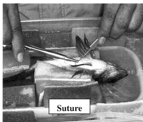
Fig. 4 An example of incised the abdomen of the rockfish and inserted the pinger.
